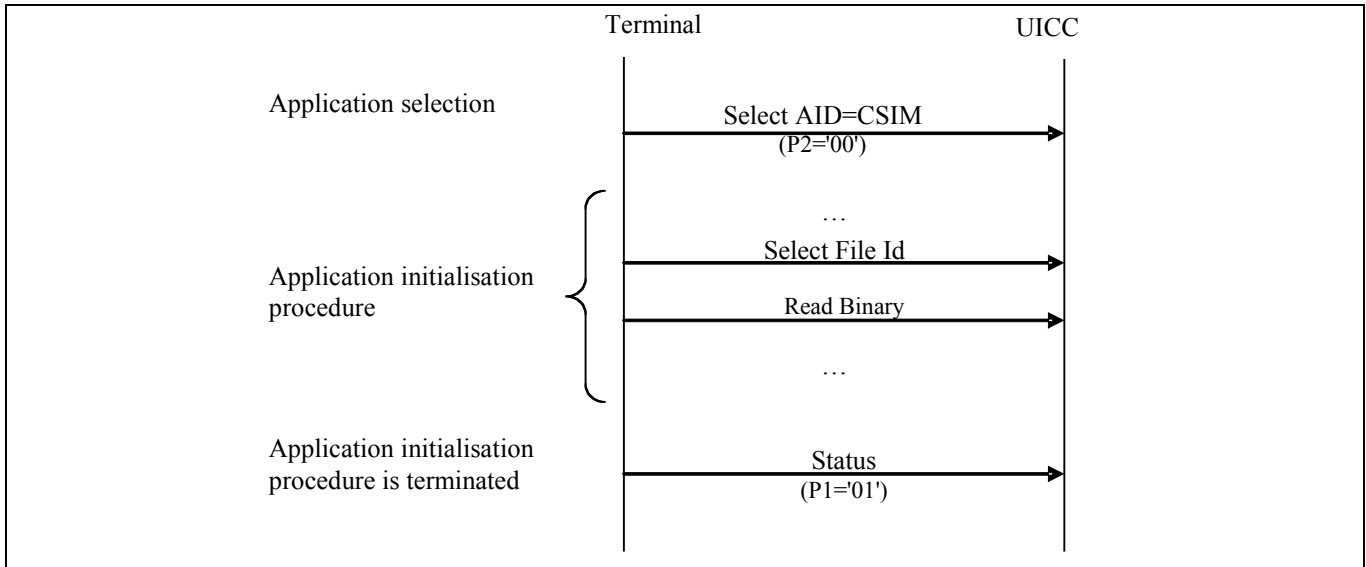
6 Figure 1 CSIM Application Session Activation Procedures
