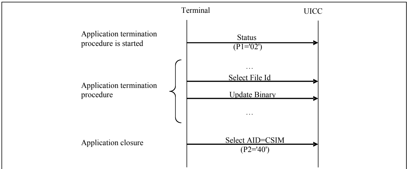
9 Figure 2 CSIM Application Session Termination Procedures
